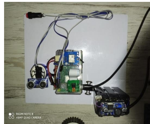
Figure 8: Hardwar
