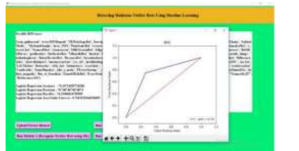
Fig.7: ROC graph
