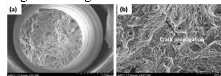
Fig 7. SEM fractography micrographs of 60µm horizontal built
