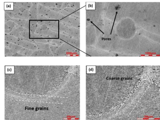
Figure 4. Optical images of AlSi10Mg @ 60 micrometers layer thickness (a) microstructure @ 200X (b) Microstructure @ 693X magnification and (c) Microstructure @ 2000X magnification (d) microstructure @ 4000X
