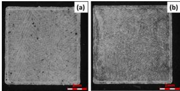
Figure 3. Top view of micro structure of AM built AlSi10Mg (a) 60 micrometers (b) 30 micrometers
