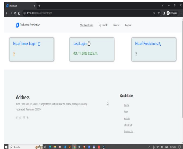
User's Dashboard
