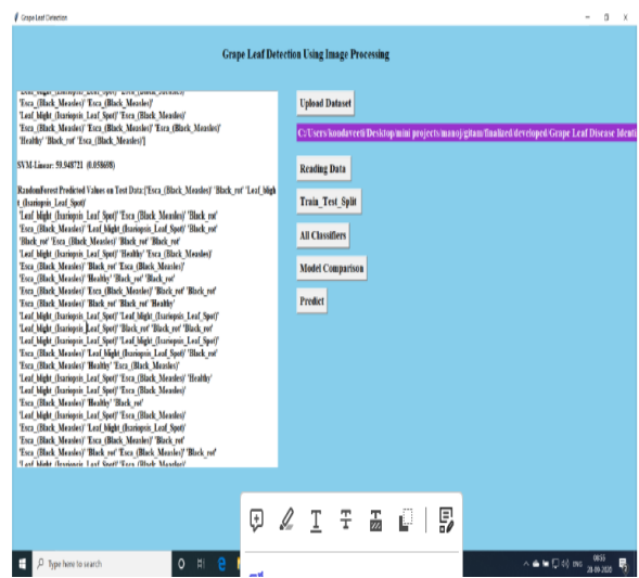
RUN ALGORITHMS
