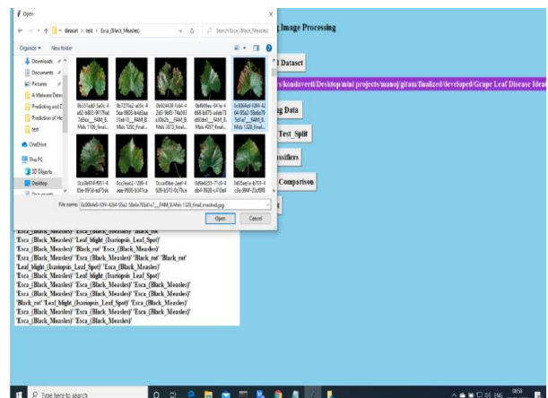
PREDICT
