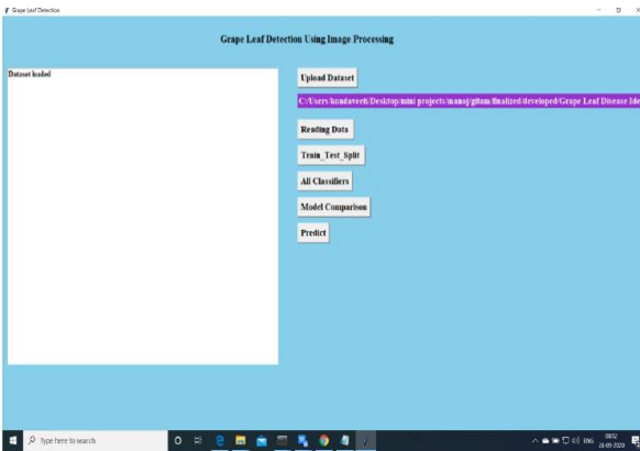
UPLOAD DATASET
