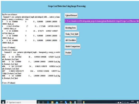
READING DATA
