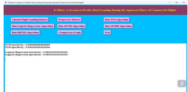
Fig.6. Output of Logistic Regression.
