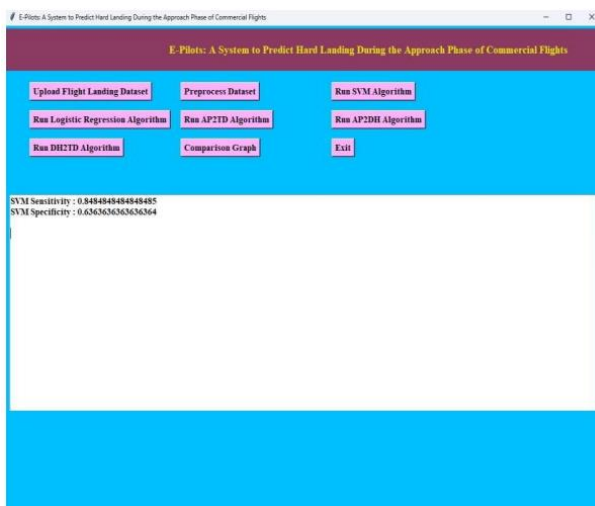
Fig.5. output of SVM.
