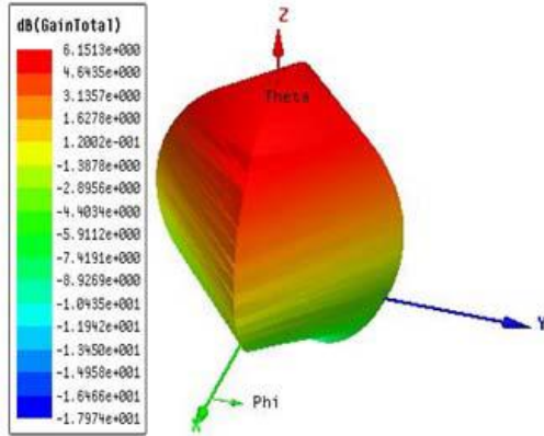
Fig.5 Simulated 3D Radiation pattern of the proposed antenna at 2.46GHz
