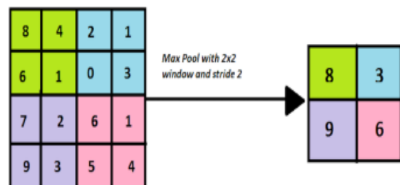
FIGURE 6: Maxpool Function
