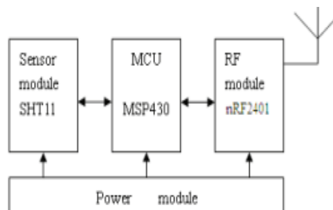
Fig.2. The hardware structure of sensor
