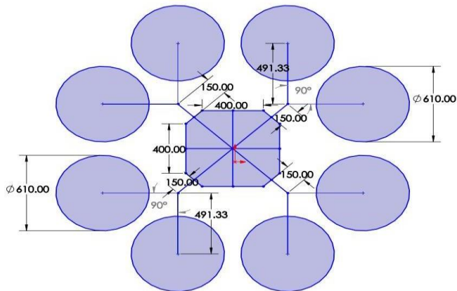
Fig -13: 2D Drawing
