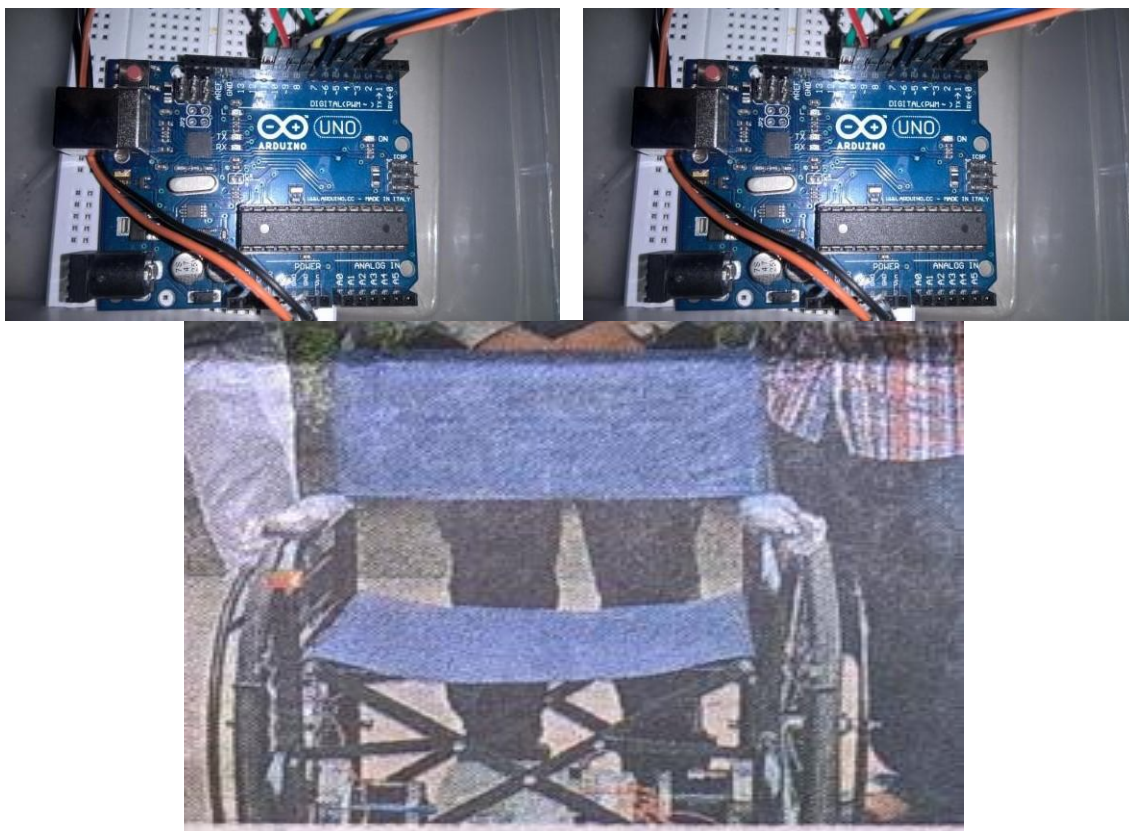
Fig-4: Model Voice Controlled Wheel Chair Via Bluetooth Mobile Application
