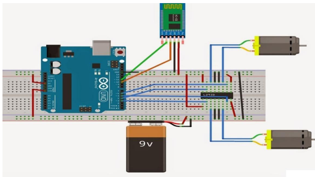
Fig- 2: Main Circuit
