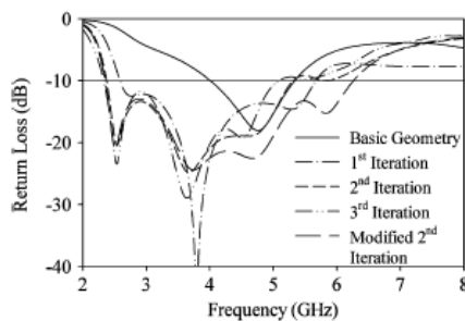
Fig. 3. Simulated return loss of the CPW-fed Koch slot antenna (without the tuning slot)
