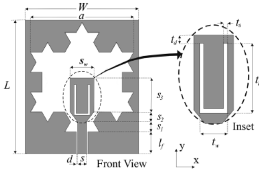
Fig. 1. Proposed slot loaded modified Koch snowflake slot antenna.
