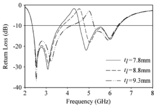
Fig. 6. Return loss of the antenna for different slot lengths
