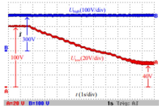
Fig. 14 The output voltage and the wide-range changed input voltage from 100V to 40V in the step-up mode.
