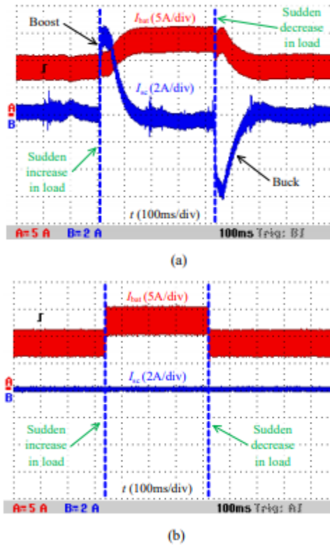
Fig. 20 Experimental results of bidirectional power flow control. (a) Super-capacitors are taken into operation. (b) Super-capacitors are not taken into operation.
