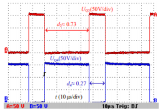
Fig. 15 The PWM voltages of power semiconductors Q3 and Q4.
