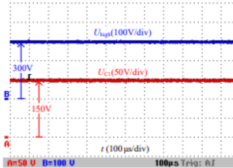
Fig. 12 Voltages across C1 and Chigh under U_{low}=40V and U_{high}=300V .
