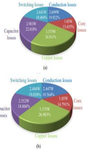
Fig. 22 Calculated power loss distributions for the experiment when U_{low}=40V , U_{high}=300V , and P_n=300W . (a) In step-up mode. (b) In step-down mode.
