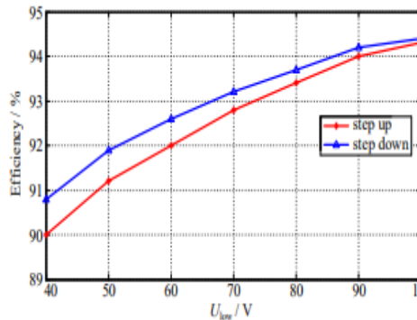
Fig. 21 Efficiencies of the proposed switched-capacitor bidirectional converter in step-up and step-down modes ( U_{high}=300V , U_{low}=40V\sim 100V , P_n=300W ).
