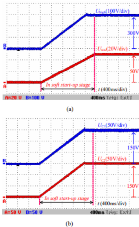
Fig. 10 Experimental results of the soft start-up. (a) The input voltage U_{low} and the output voltage U_{high} . (b) The voltages across C1 and C2.
