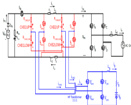
Fig. 2. Detailed Schematic of Proposed MZSI inductor current during the shoot-through time interval D_{0T}/2\pi as follow [8]:
