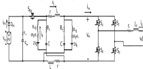
Fig. 4. Equivalent Model of the proposed Modified Z-source Inverter (MZSI) with battery From equation (12)-(15), state space equations for the entire system can be written as:
