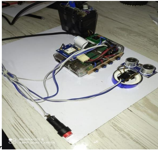
Figure 8: Hardware Setup
