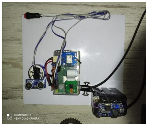
Figure 7: Implementation of Hardware Setup
