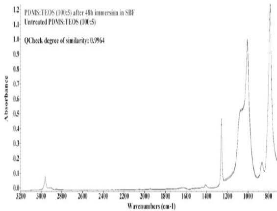
Figure 9 shows a comparison between the FT-IR spectra of untreated PDMS: TEOS (100:5) and PDMS: TEOS (100:5) that was immersed in SBF for 48 hours.
