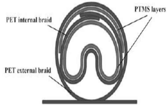
Figure 6. TPAM with an overlap
