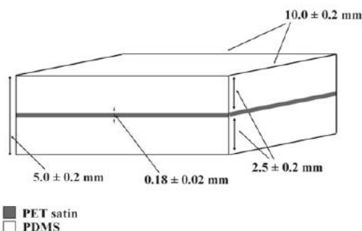
Figure 3. Shape of sample for biocompatibility tests
