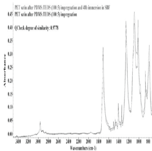
FT-IR spectra of PET satin before and after PDMS:TEOS (100:5) impregnation and 48 hours of immersion in SBF are shown in Figure 11.
