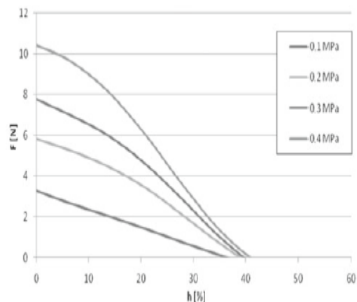
Figure 13. Static characteristic of TPAM with glued core
