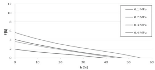
Figure 12. Static characteristic of TPAM with PDMS core
