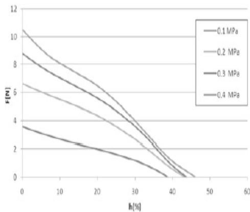
Figure 14. Static characteristic of uniform TPAM
